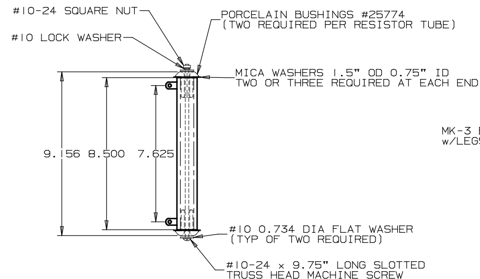
RESISTOR ASSEMBLY DETAIL
