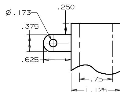
RESISTOR TERMINAL DETAIL
