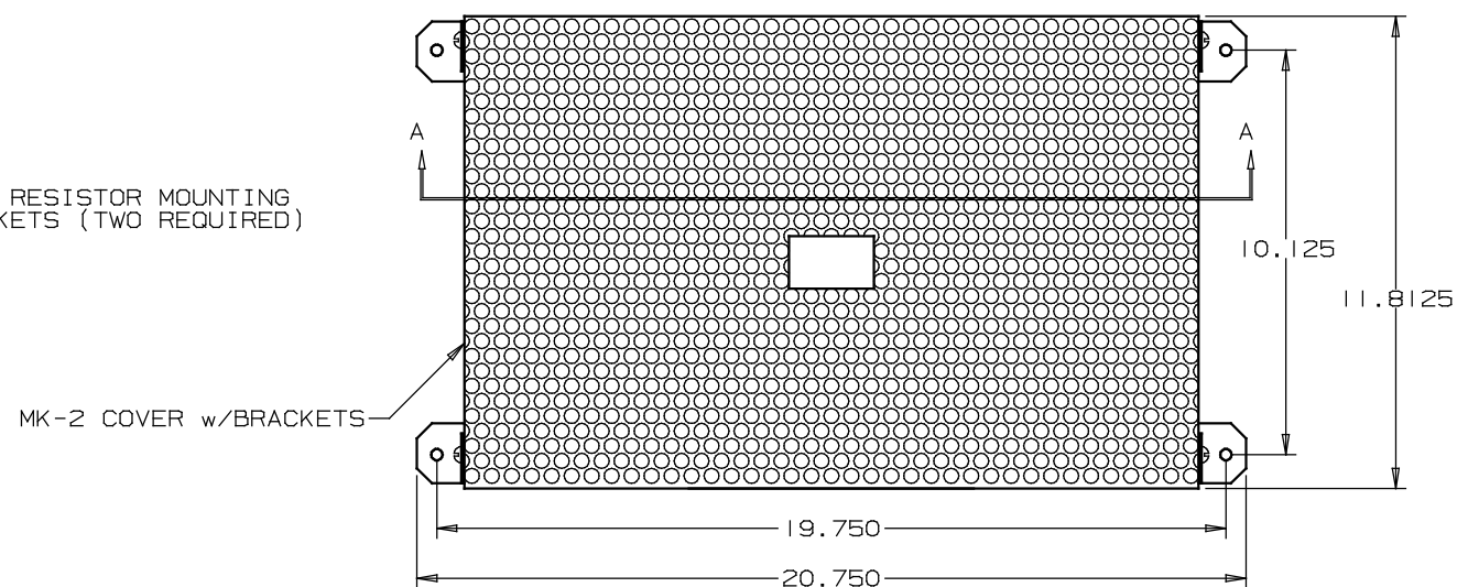
TOP VIEW
