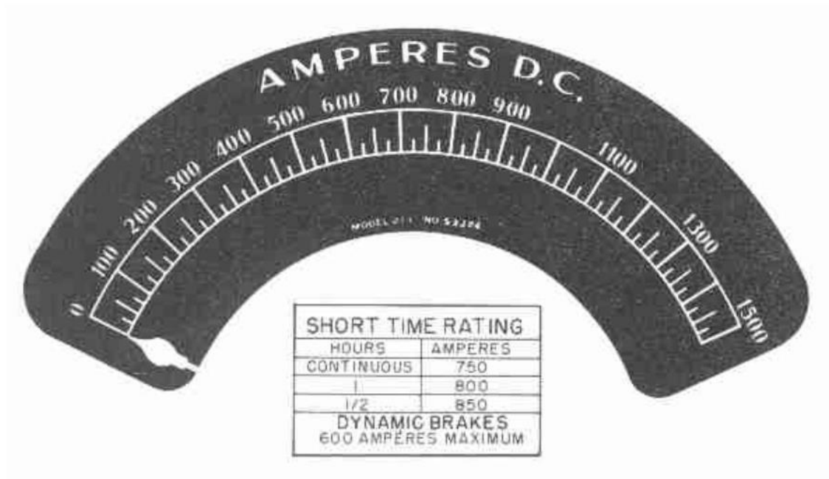
Load Indicating Meter Fig. 1-3
