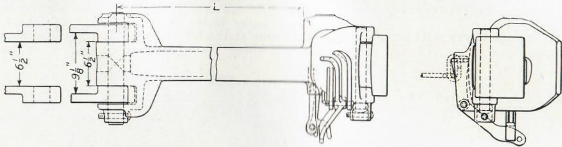
Fig. 2107—Sharon Side Operating Coupler with Shank for Quadruple Shear Pivot Pin.
