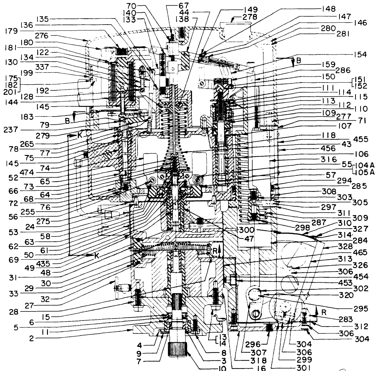
Ref. No. 1 SECTION A-A
