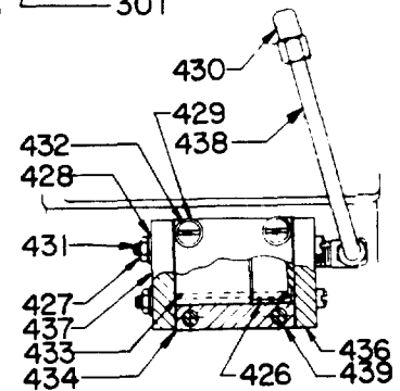
SECTION K-K Ref. No. 425
