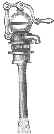
Fig. 381. WASH-ROOM PUMP.
